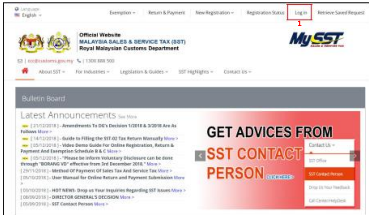
Figure 1: MySST website
